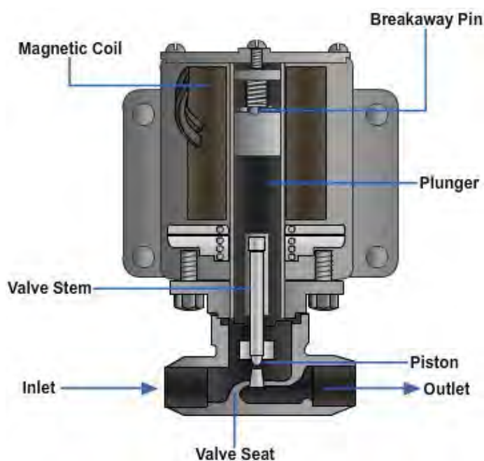
Figure 12-26 – Solenoid stop valve.
