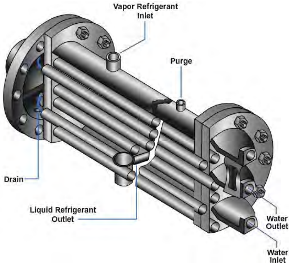
Figure 12-19 –Water-cooled condenser.
