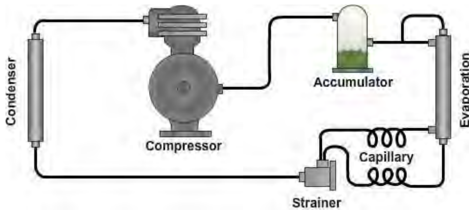
Figure 12-31 —Accumulator location.
