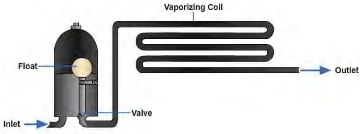
Figure 12-23 – High-side float expansion valve.
