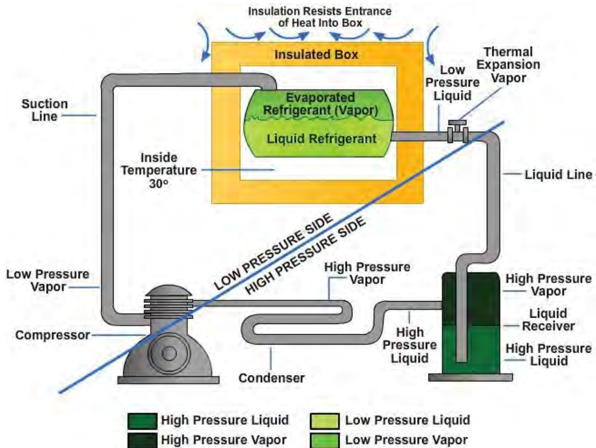
Figure 12-12 – Refrigeration cycle.
