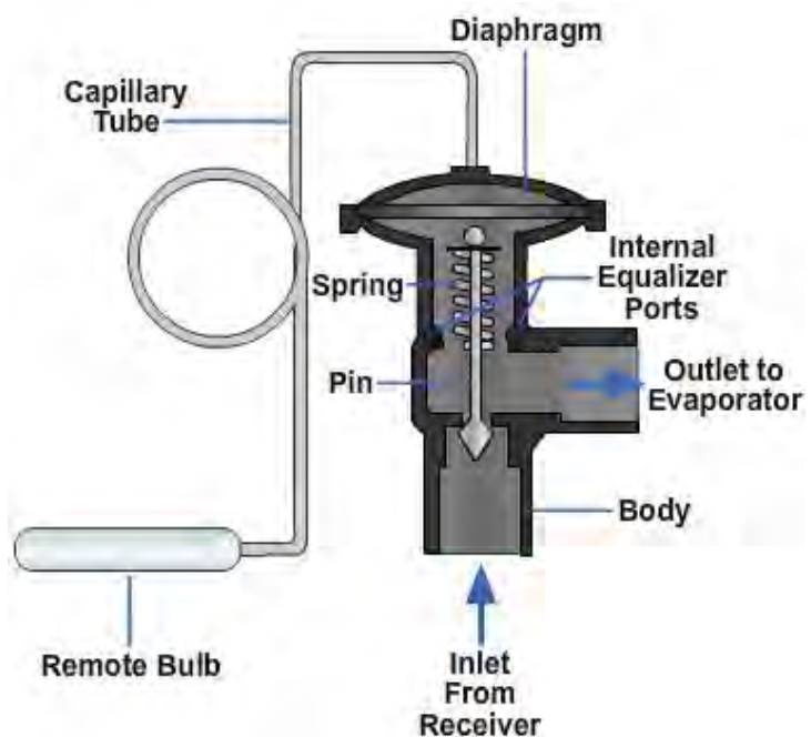
Figure 12-21 - Thermostatic expansion valve.
