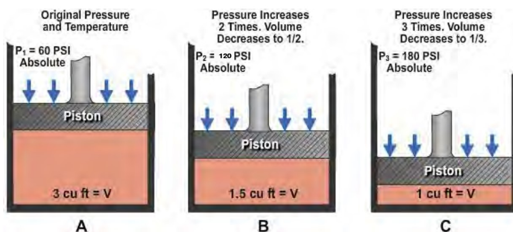
Figure 12-5 – Pressure-volume relationship.
